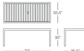
RECTANGULAR DINING TABLE MRT303 w:78.75" d:35.5" h:30" Seat Height: N/A Arm Height: N/A Weight: 60 lbs.
