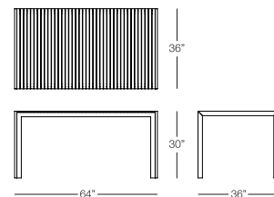
RECTANGULAR DINING TABLE SIC306 w:64" d:36" h:30" Seat Height: N/A Arm Height: N/A Weight: 57 lbs.
