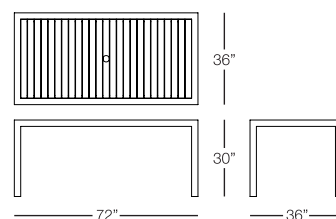
RECTANGULAR DINING TABLE with alumiwood top MAR343 w:72" d:36" h:30" Seat Height: N/A Arm Height: N/A Weight: 92 lbs.
